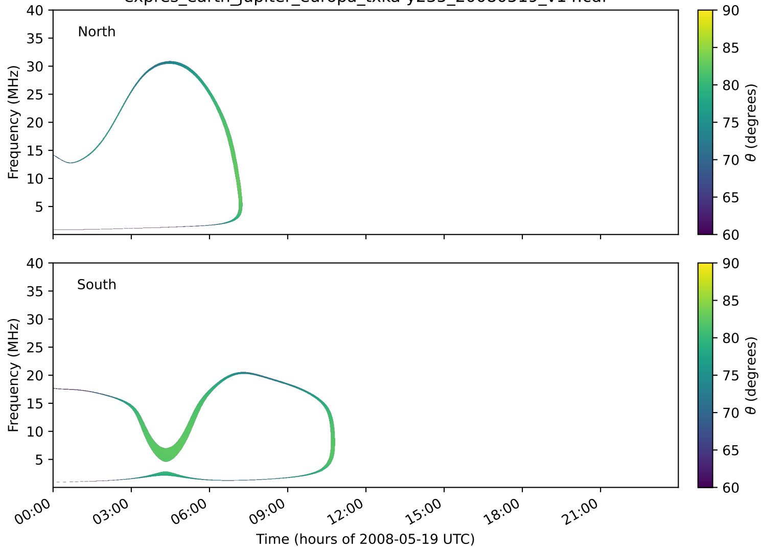
expres_earth_jupiter_europa_txka-y235_20080519_v14.cdf
