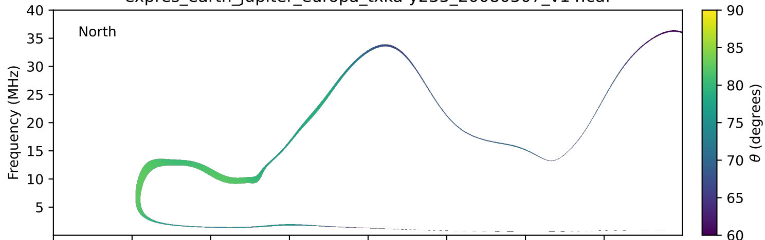
expres_earth_jupiter_europa_txka-y235_20080507_v14.cdf
