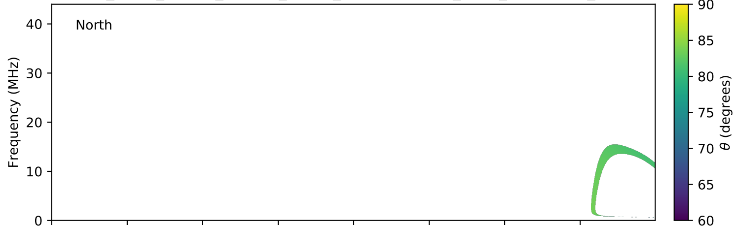
expres_earth_jupiter_europa_jrm09_lossc-wid1deg_3kev_20080524_v01.cdf
