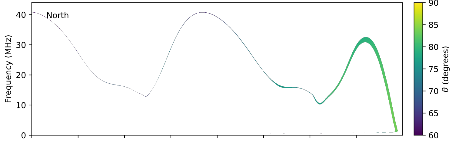
expres_earth_jupiter_europa_jrm09_lossc-wid1deg_3kev_20080522_v01.cdf
