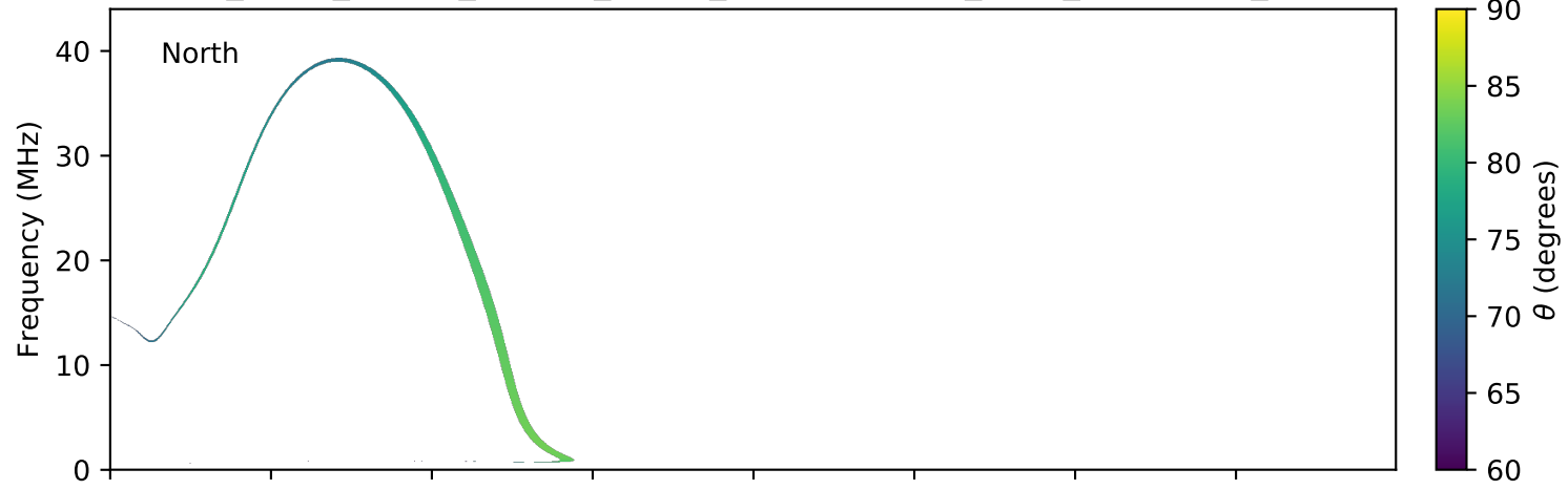
expres_earth_jupiter_europa_jrm09_lossc-wid1deg_3kev_20080519_v01.cdf
