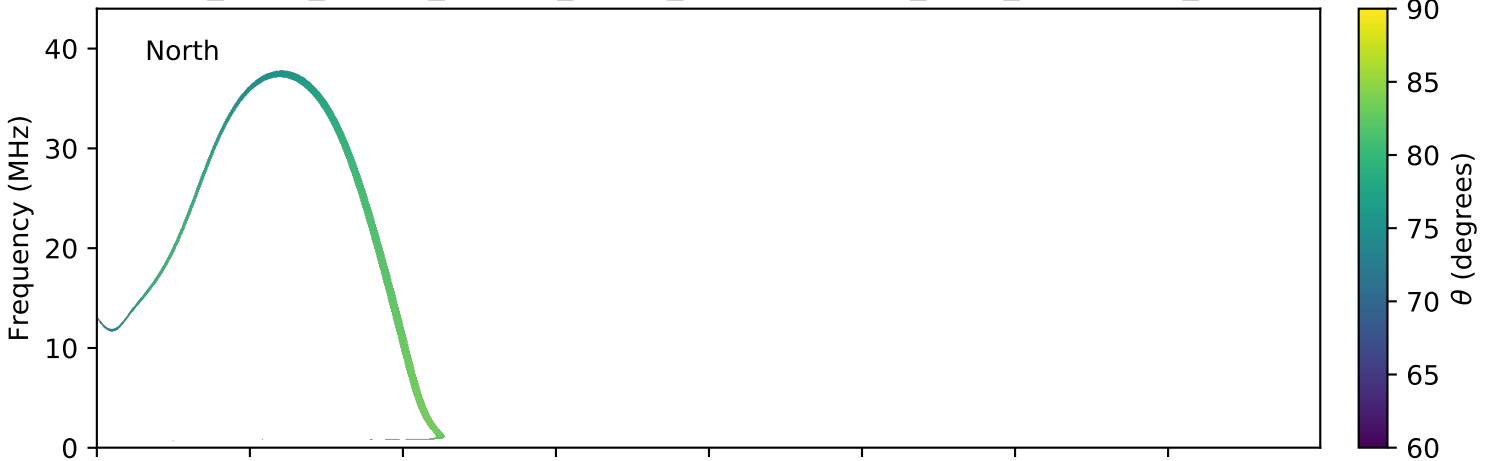
expres_earth_jupiter_europa_jrm09_lossc-wid1deg_3kev_20080512_v01.cdf
