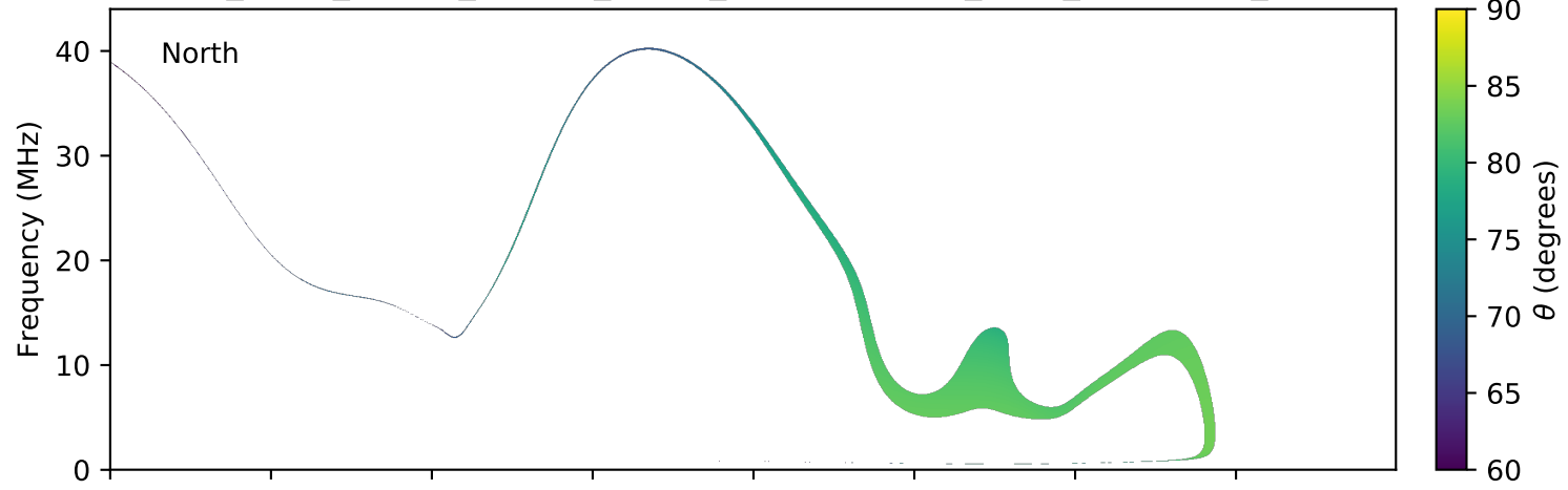
expres_earth_jupiter_europa_jrm09_lossc-wid1deg_3kev_20080508_v01.cdf
