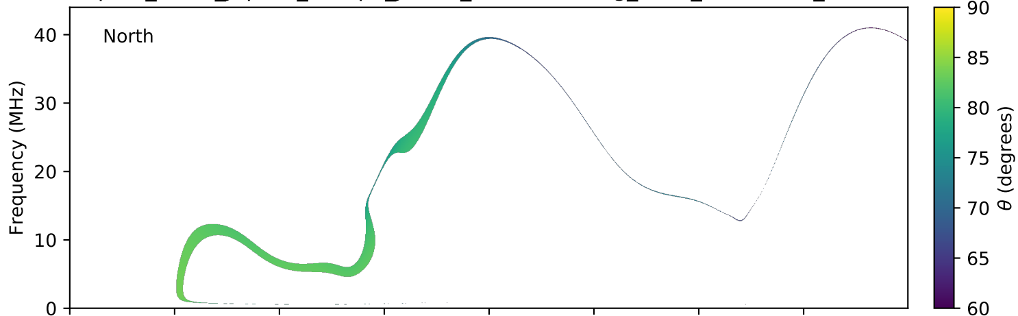
expres_earth_jupiter_europa_jrm09_lossc-wid1deg_3kev_20080507_v01.cdf
