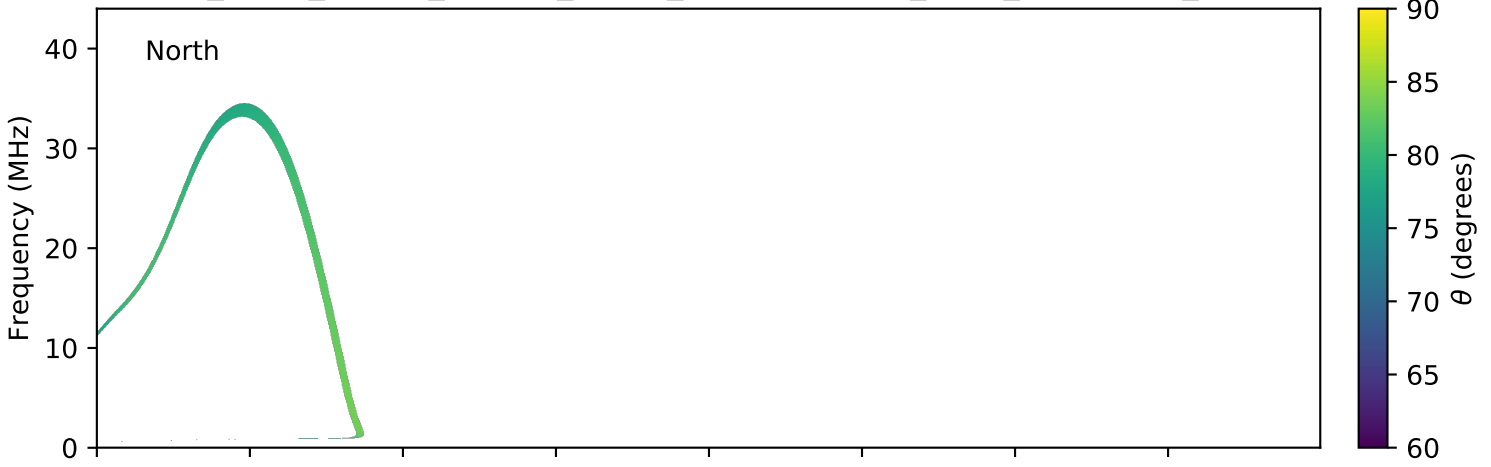
expres_earth_jupiter_europa_jrm09_lossc-wid1deg_3kev_20080505_v01.cdf
