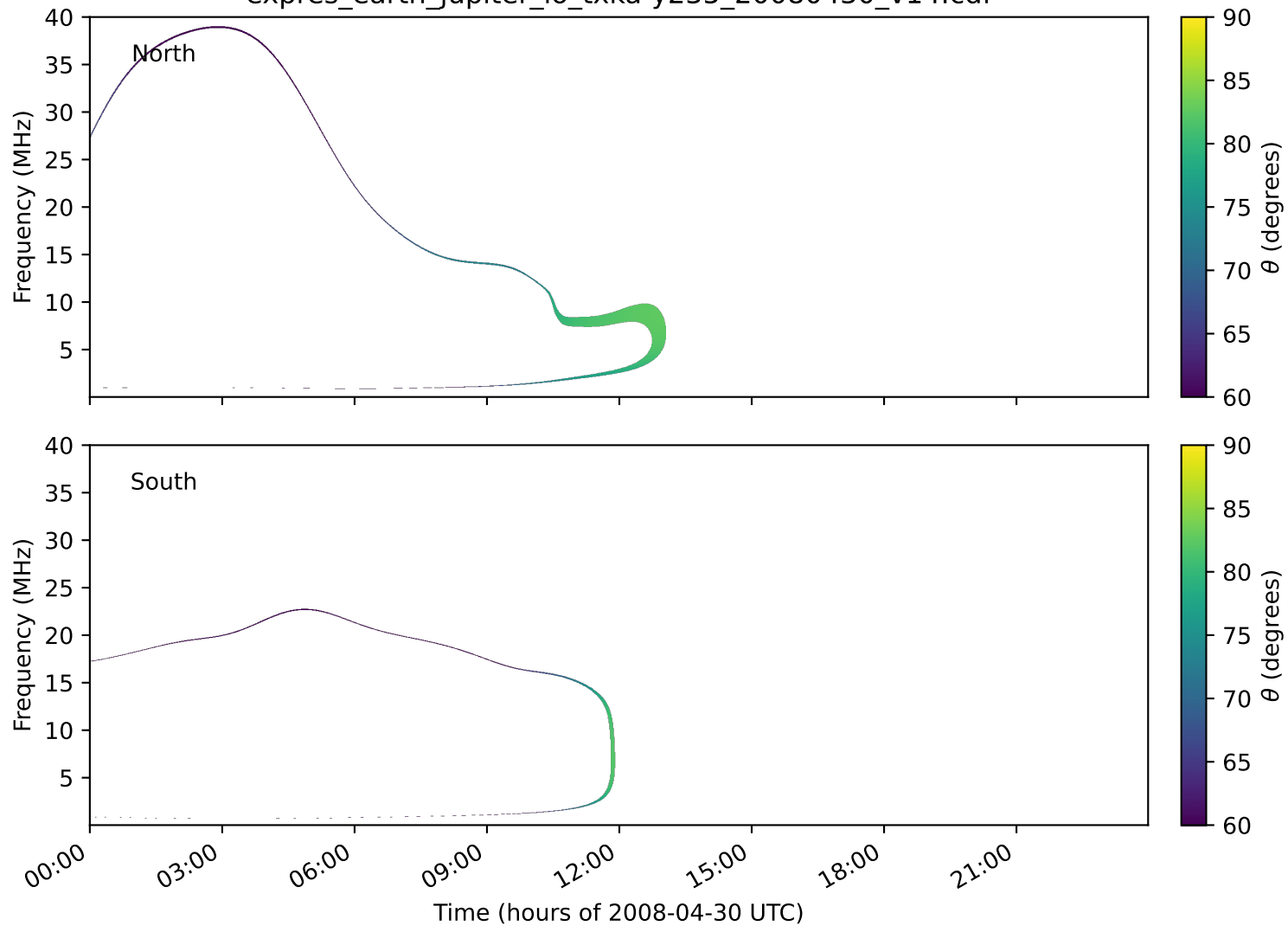
expres_earth_jupiter_io_txka-y235_20080430_v14.cdf
