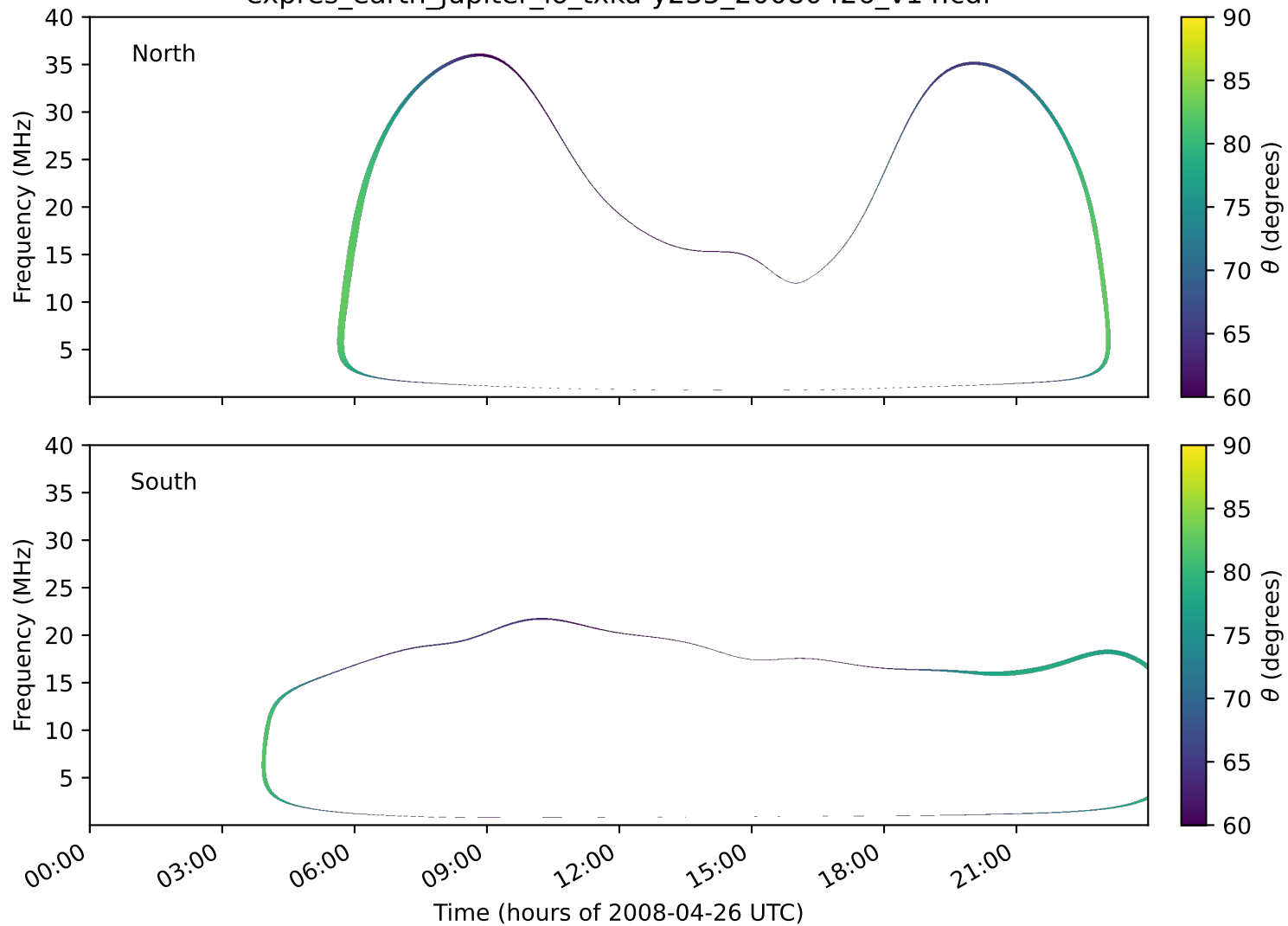
expres_earth_jupiter_io_txka-y235_20080426_v14.cdf
