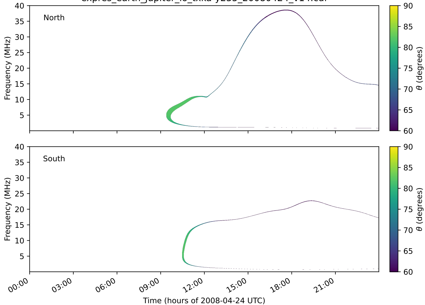
expres_earth_jupiter_io_txka-y235_20080424_v14.cdf
