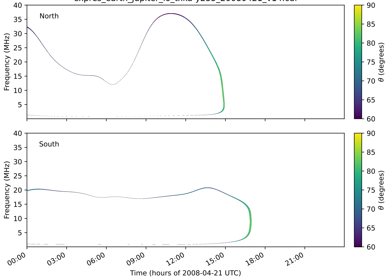
expres_earth_jupiter_io_txka-y235_20080421_v14.cdf
