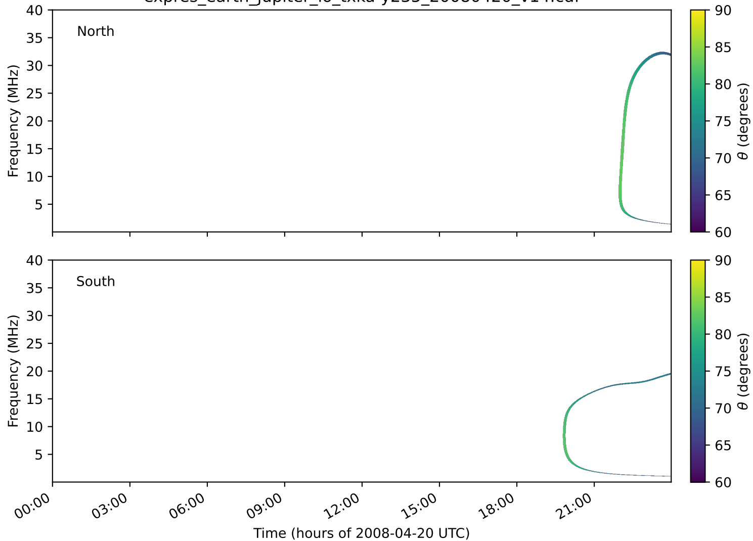
expres_earth_jupiter_io_txka-y235_20080420_v14.cdf
