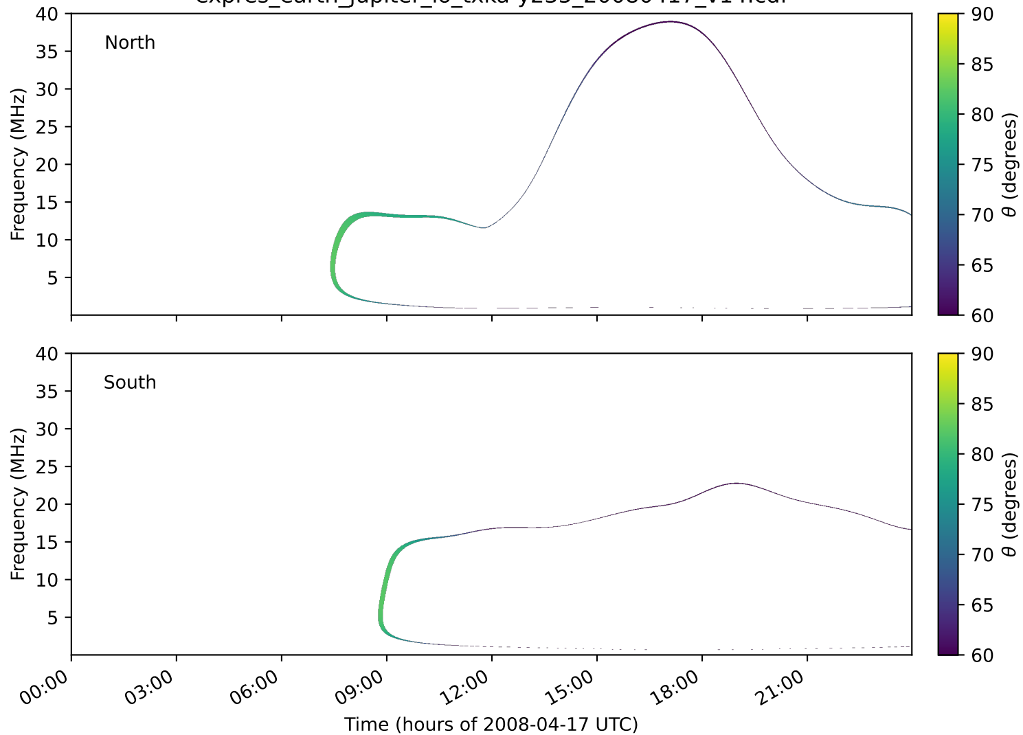
expres_earth_jupiter_io_txka-y235_20080417_v14.cdf
