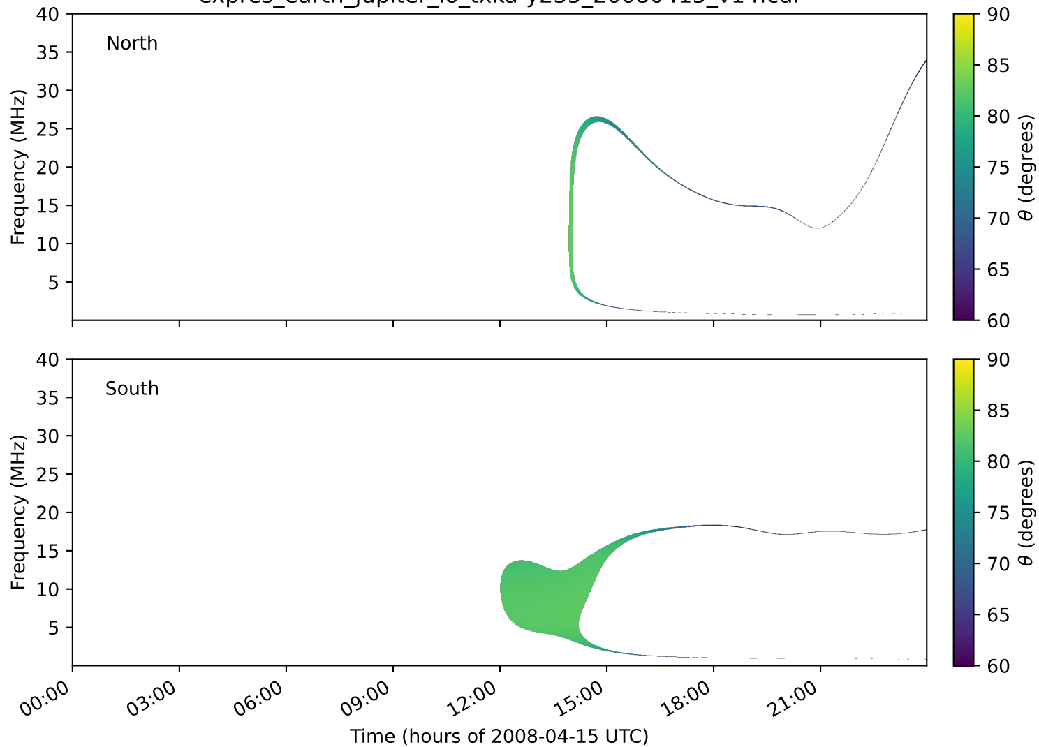
expres_earth_jupiter_io_txka-y235_20080415_v14.cdf
