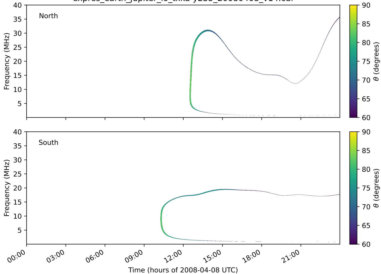
expres_earth_jupiter_io_txka-y235_20080408_v14.cdf
