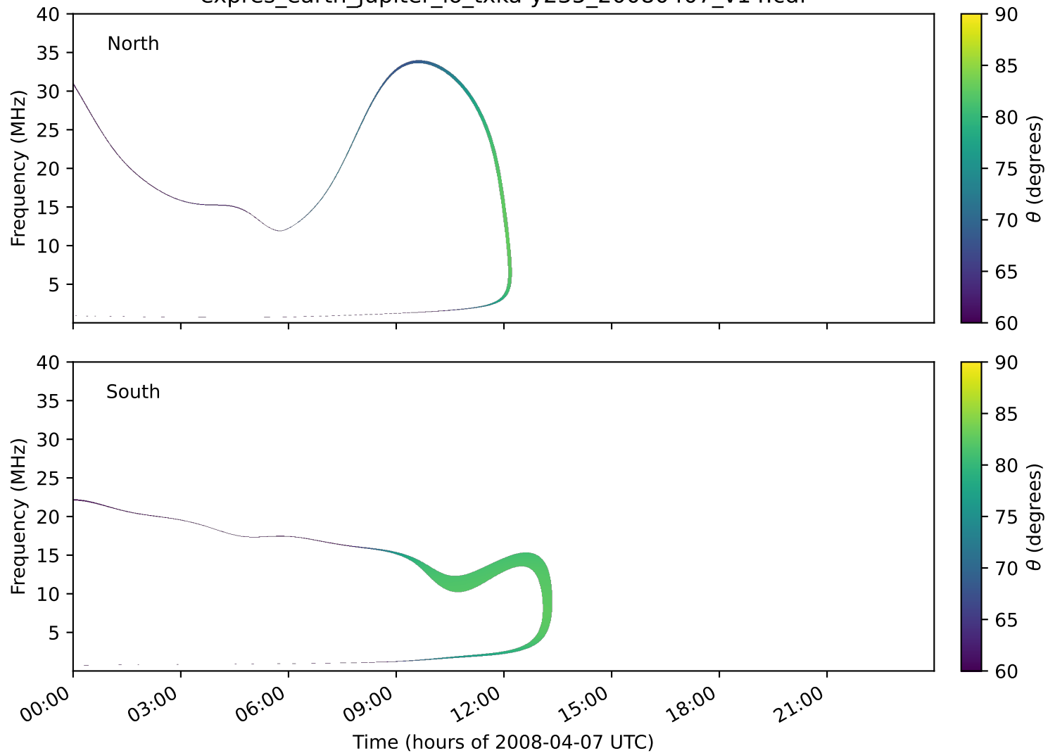
expres_earth_jupiter_io_txka-y235_20080407_v14.cdf
