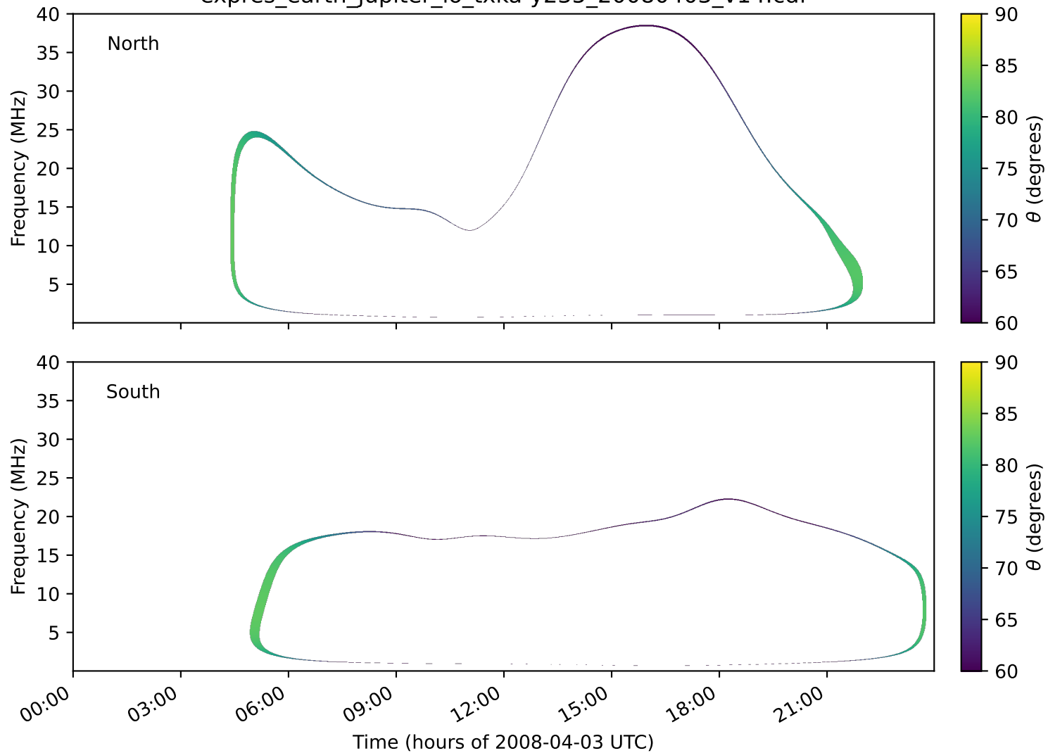
expres_earth_jupiter_io_txka-y235_20080403_v14.cdf
