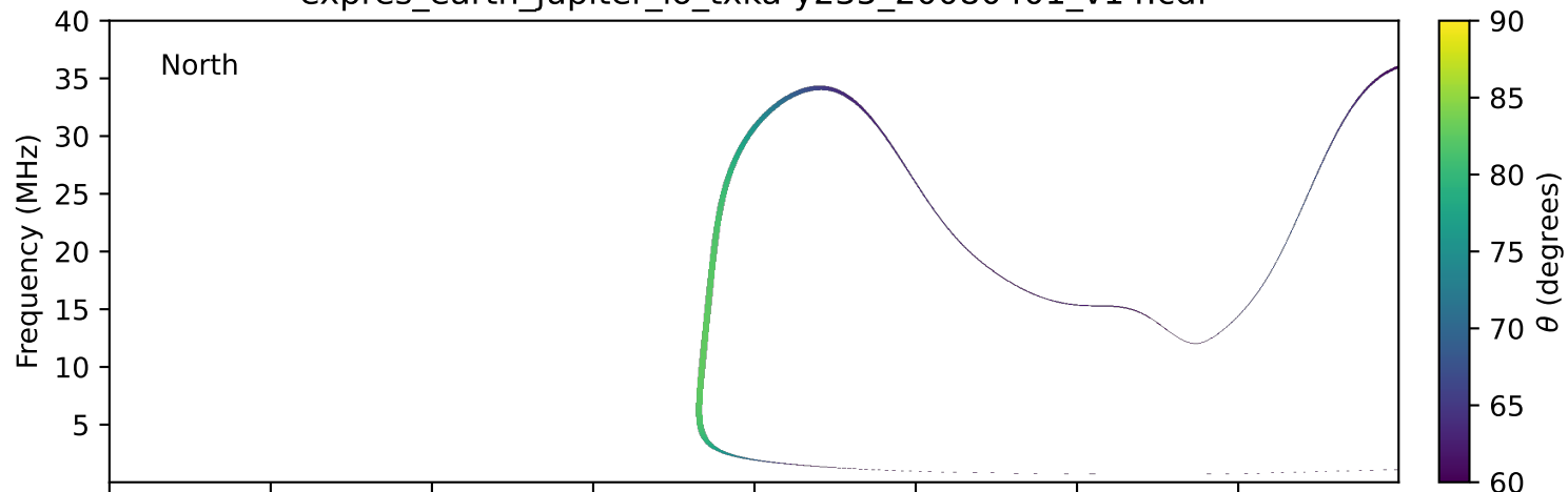
expres_earth_jupiter_io_txka-y235_20080401_v14.cdf
