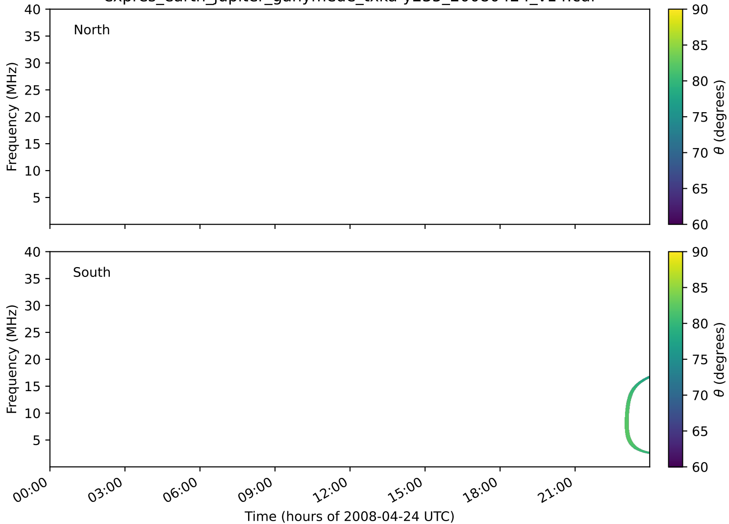
expres_earth_jupiter_ganymede_txka-y235_20080424_v14.cdf
