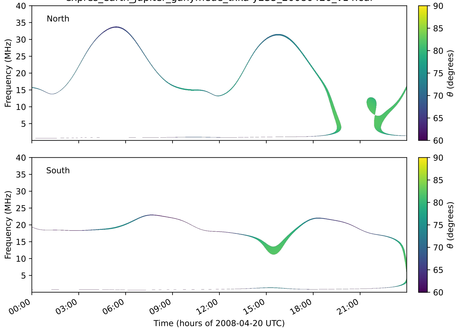
expres_earth_jupiter_ganymede_txka-y235_20080420_v14.cdf
