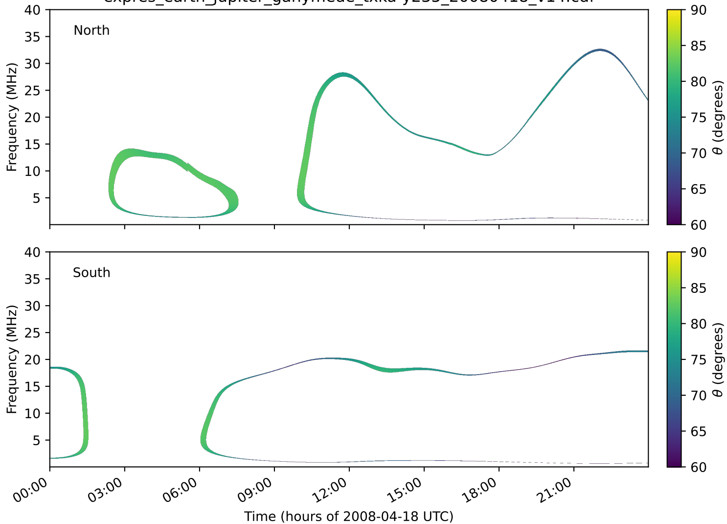
expres_earth_jupiter_ganymede_txka-y235_20080418_v14.cdf
