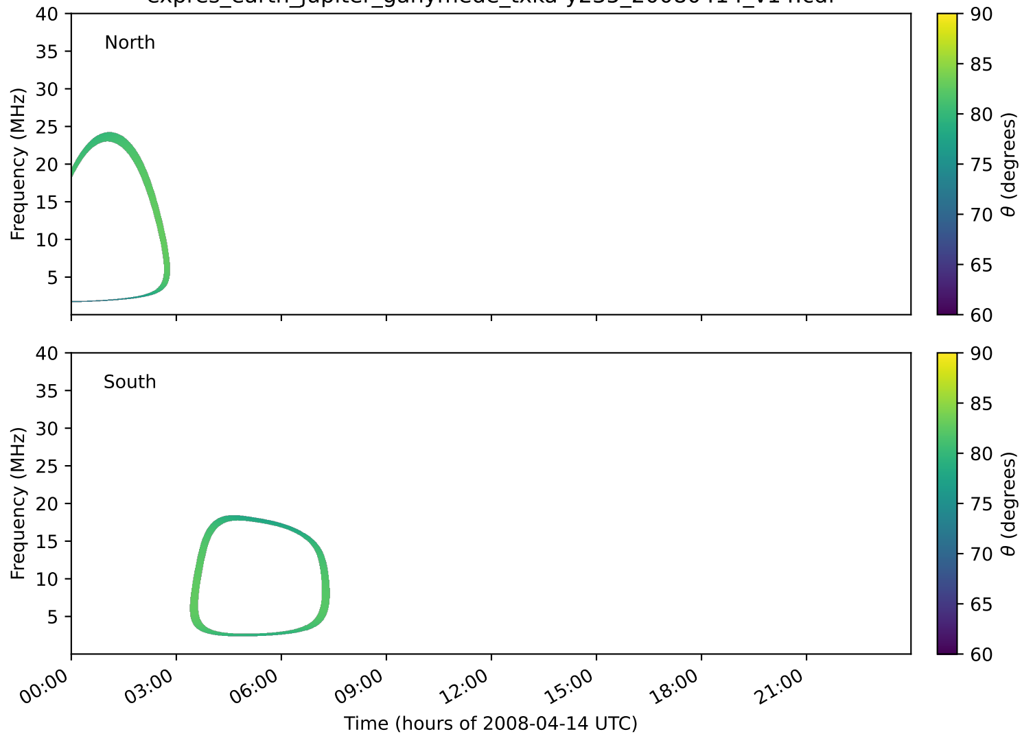
expres_earth_jupiter_ganymede_txka-y235_20080414_v14.cdf
