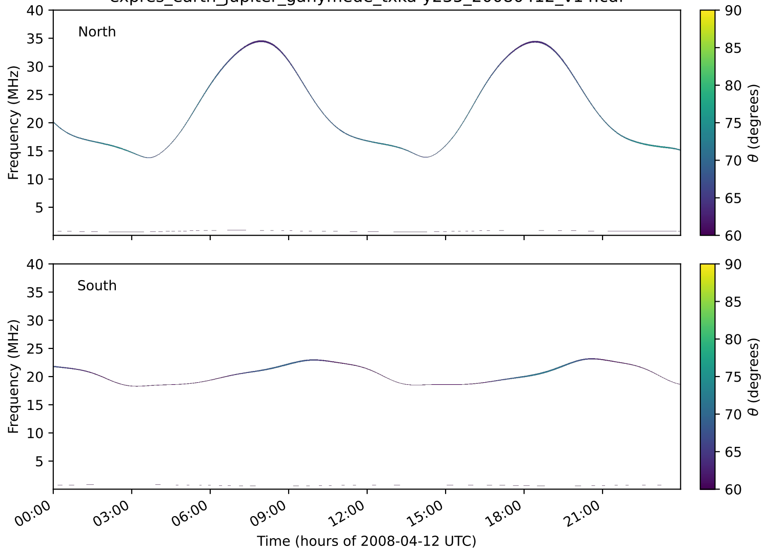
expres_earth_jupiter_ganymede_txka-y235_20080412_v14.cdf
