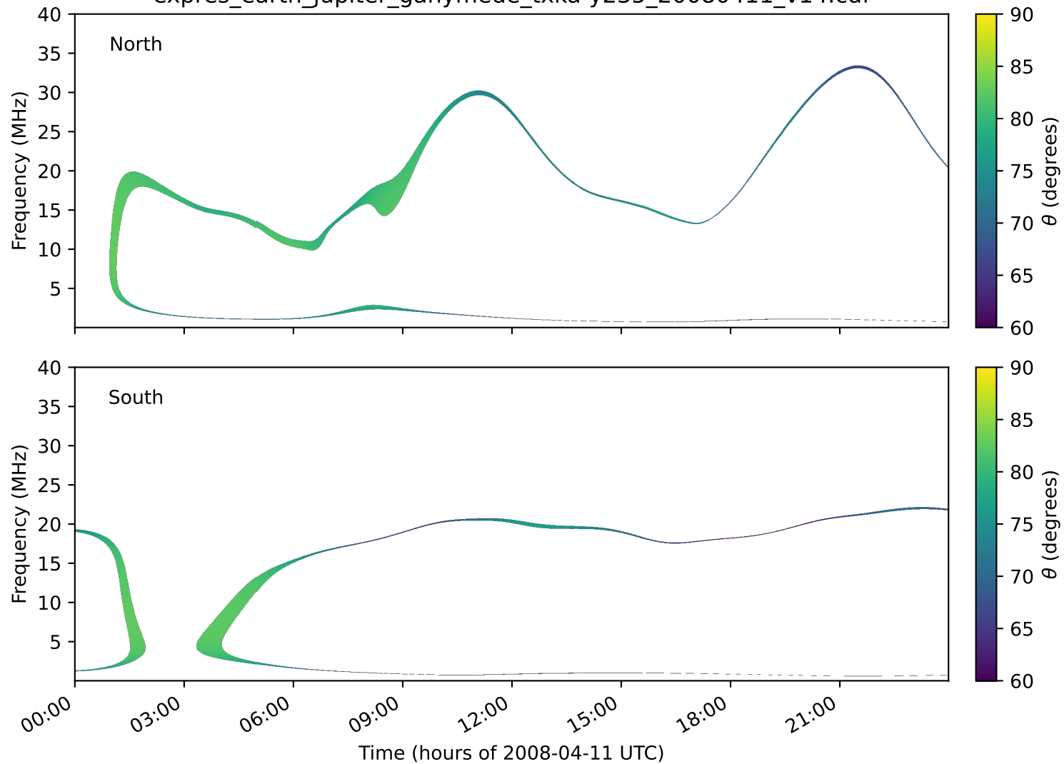
expres_earth_jupiter_ganymede_txka-y235_20080411_v14.cdf
