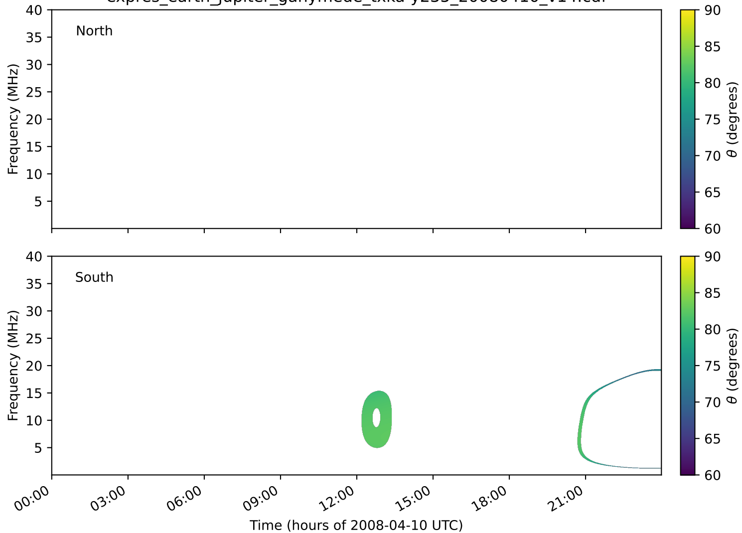
expres_earth_jupiter_ganymede_txka-y235_20080410_v14.cdf
