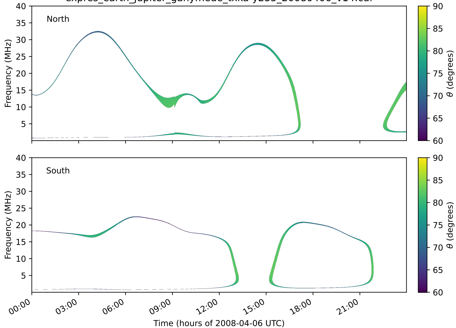
expres_earth_jupiter_ganymede_txka-y235_20080406_v14.cdf
