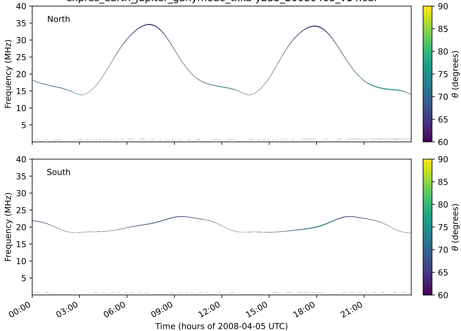
expres_earth_jupiter_ganymede_txka-y235_20080405_v14.cdf
