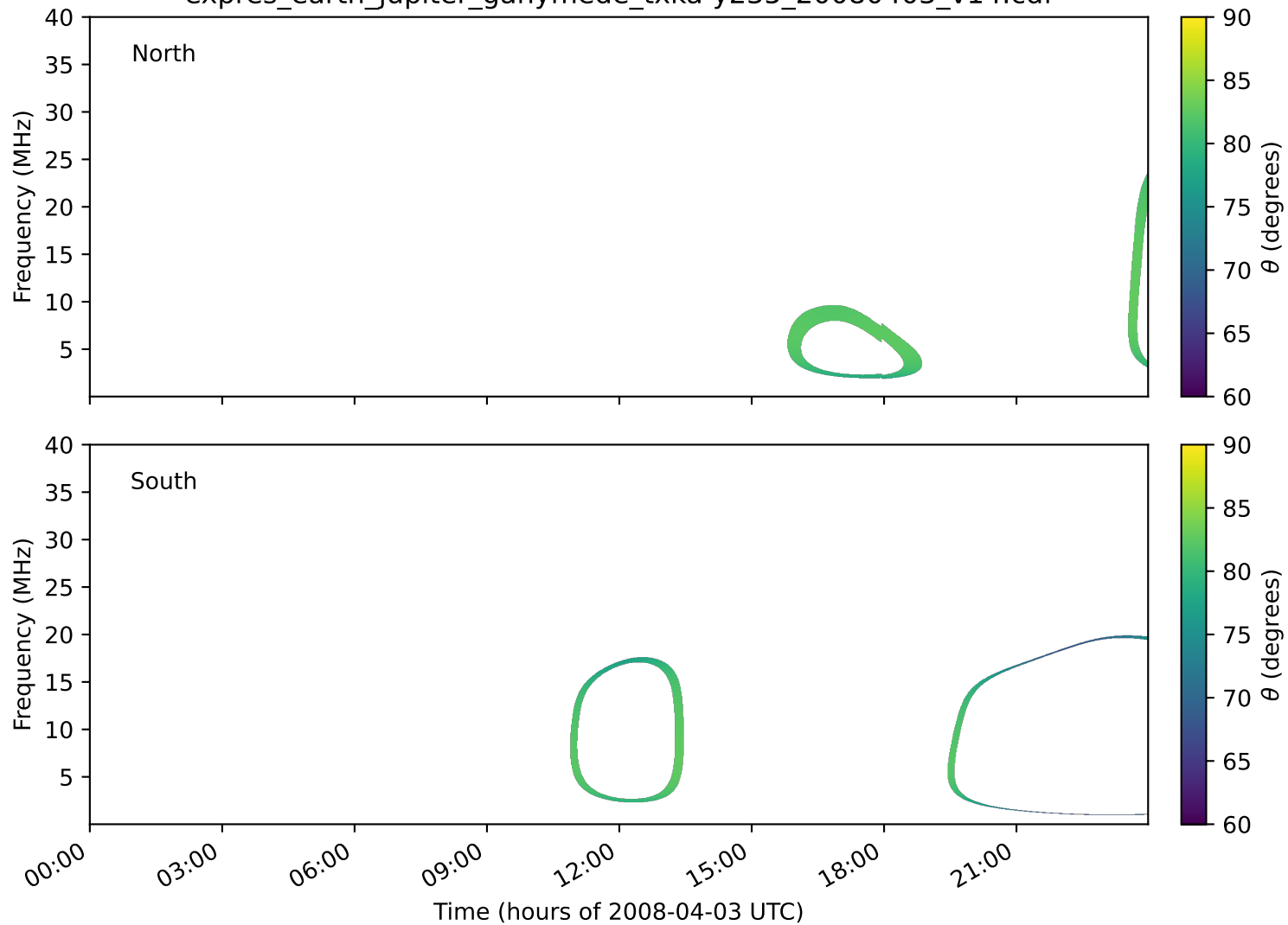
expres_earth_jupiter_ganymede_txka-y235_20080403_v14.cdf
