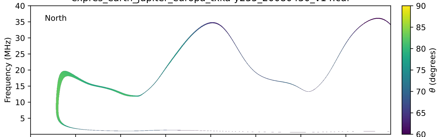
expres_earth_jupiter_europa_txka-y235_20080430_v14.cdf
