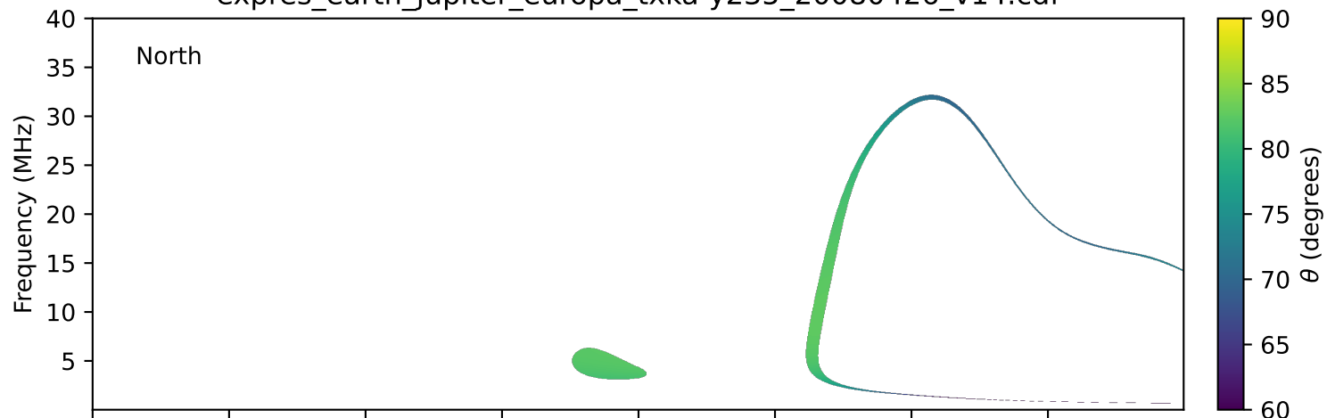
expres_earth_jupiter_europa_txka-y235_20080426_v14.cdf
