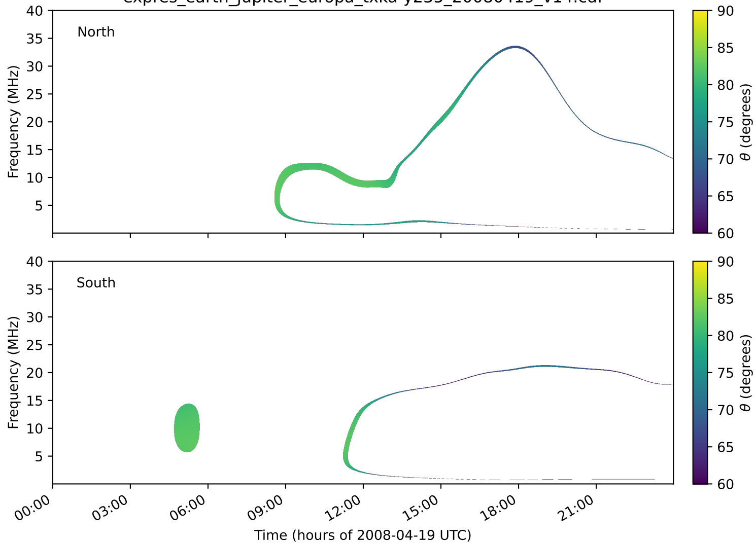
expres_earth_jupiter_europa_txka-y235_20080419_v14.cdf
