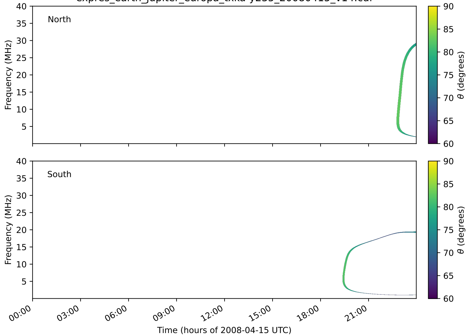
expres_earth_jupiter_europa_txka-y235_20080415_v14.cdf
