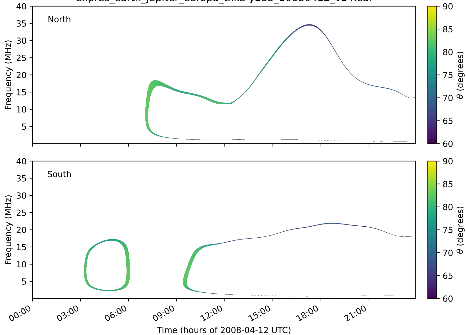
expres_earth_jupiter_europa_txka-y235_20080412_v14.cdf
