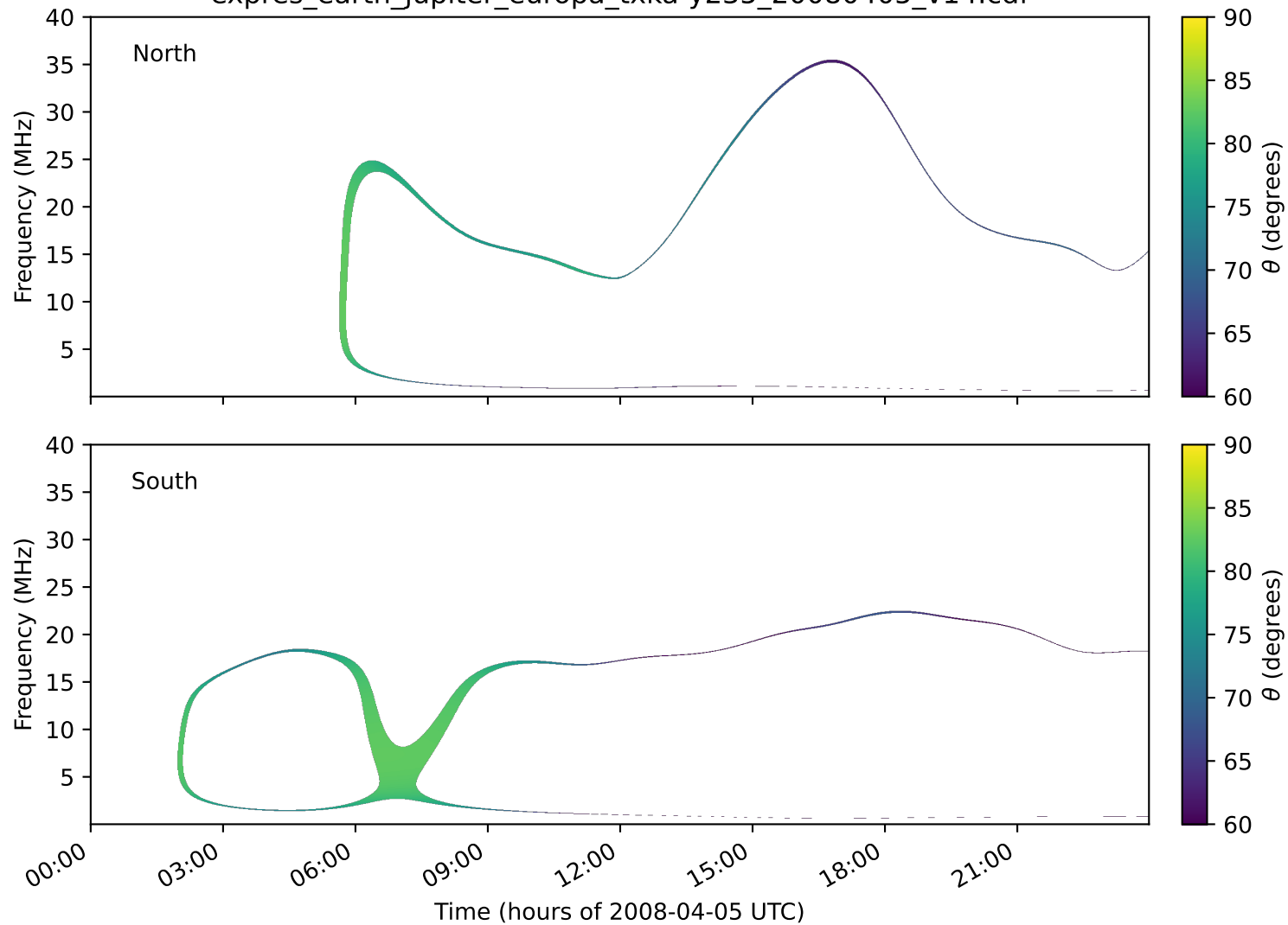
expres_earth_jupiter_europa_txka-y235_20080405_v14.cdf
