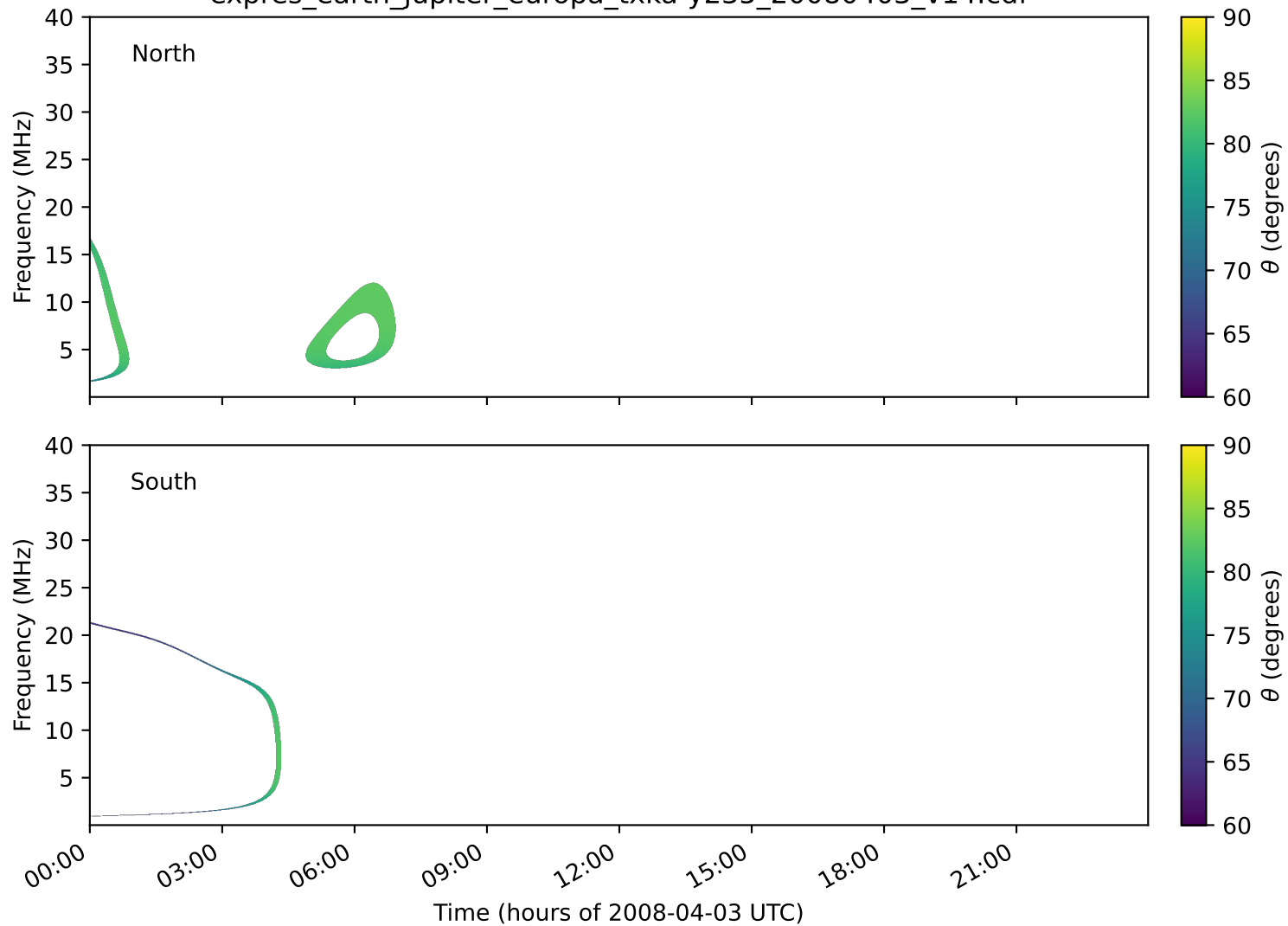
expres_earth_jupiter_europa_txka-y235_20080403_v14.cdf
