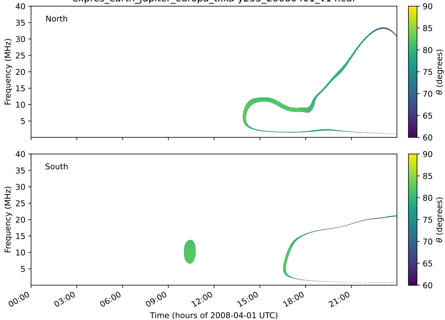
expres_earth_jupiter_europa_txka-y235_20080401_v14.cdf
