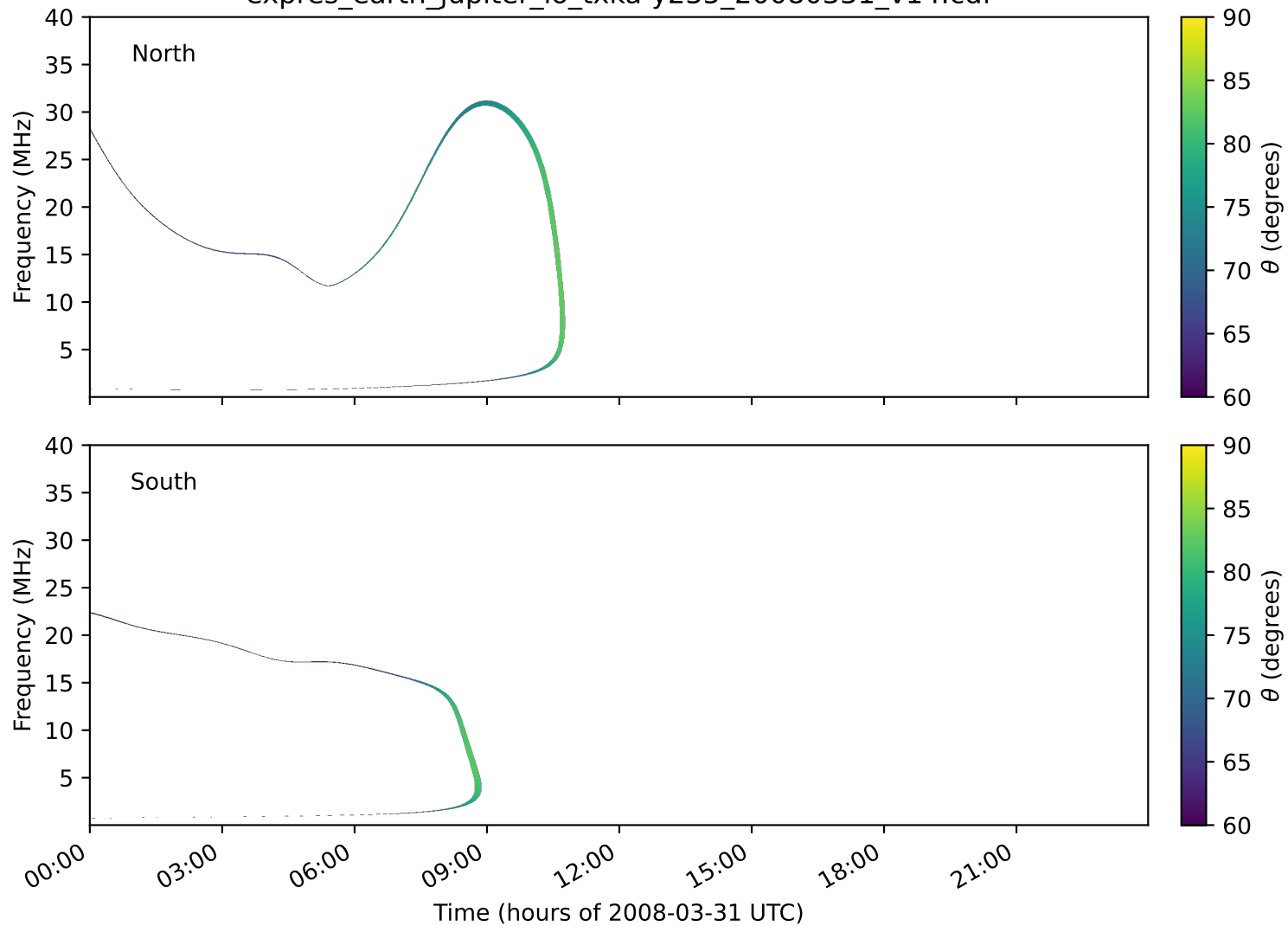
expres_earth_jupiter_io_txka-y235_20080331_v14.cdf
