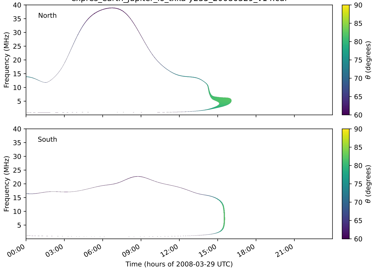
expres_earth_jupiter_io_txka-y235_20080329_v14.cdf
