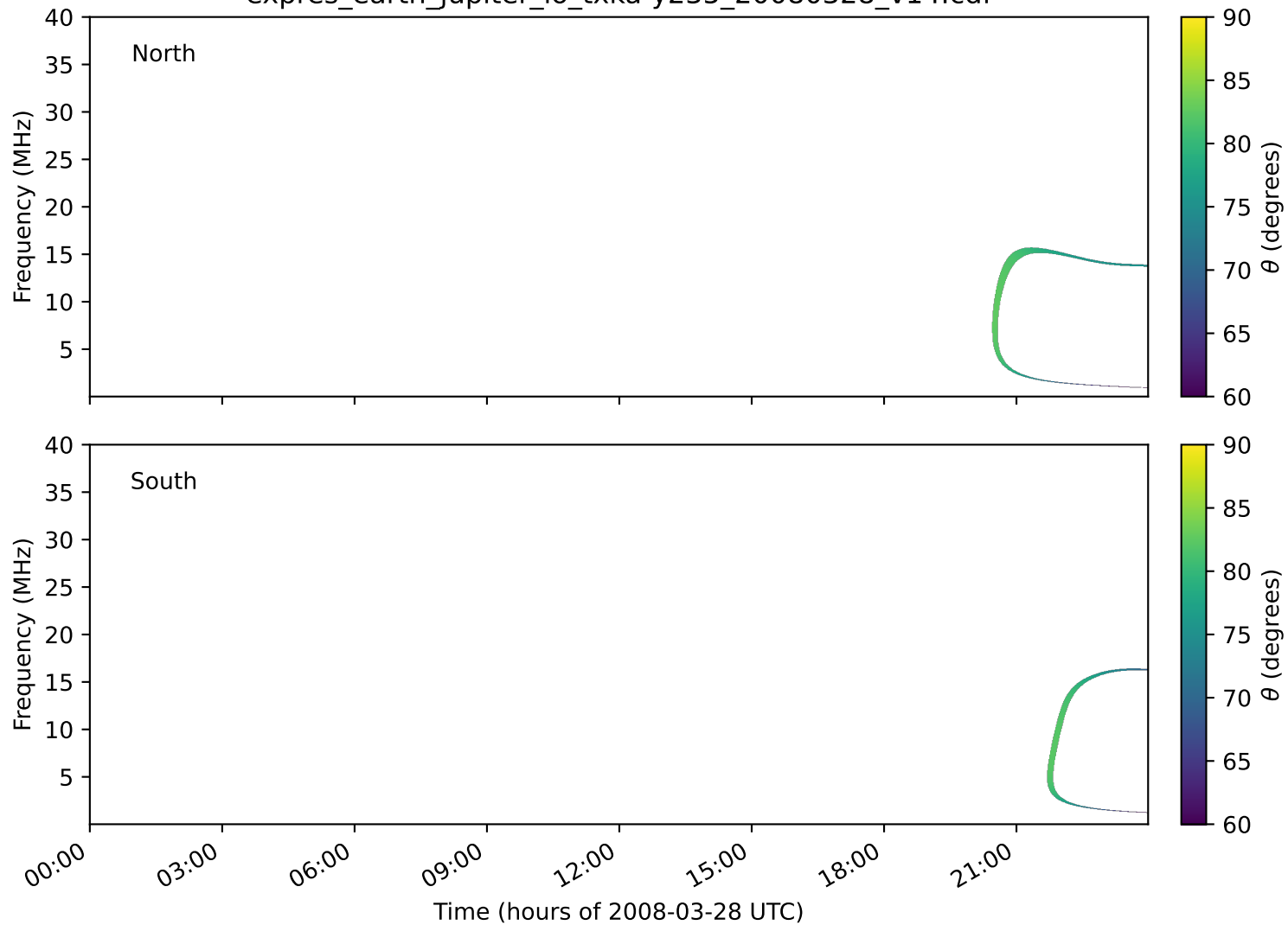
expres_earth_jupiter_io_txka-y235_20080328_v14.cdf
