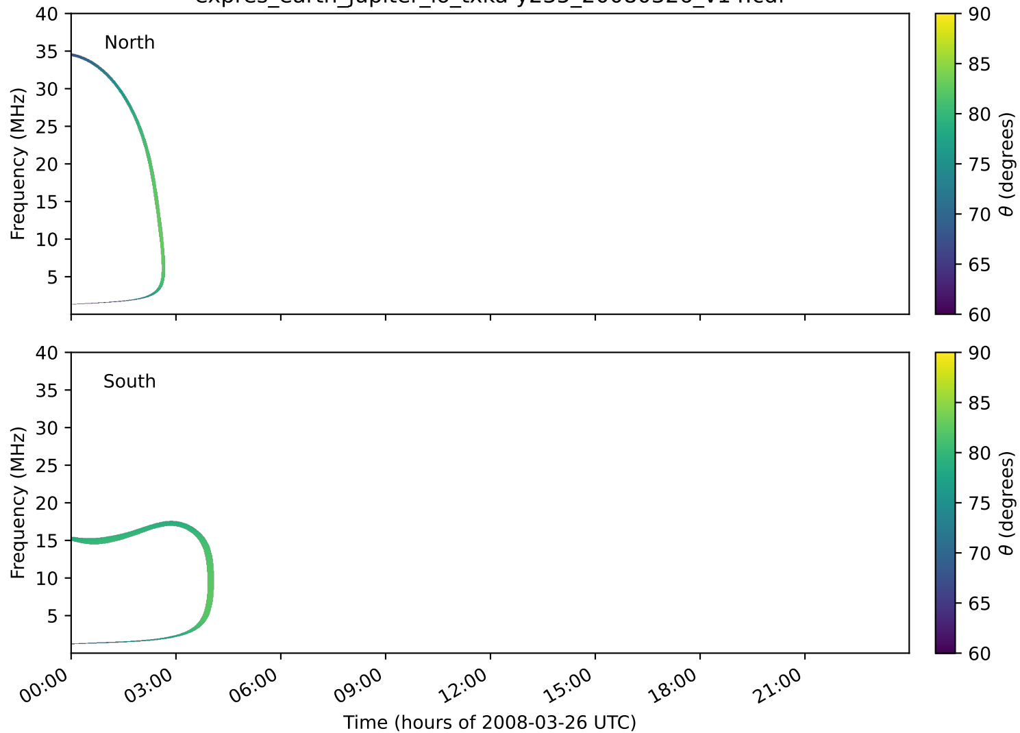
expres_earth_jupiter_io_txka-y235_20080326_v14.cdf
