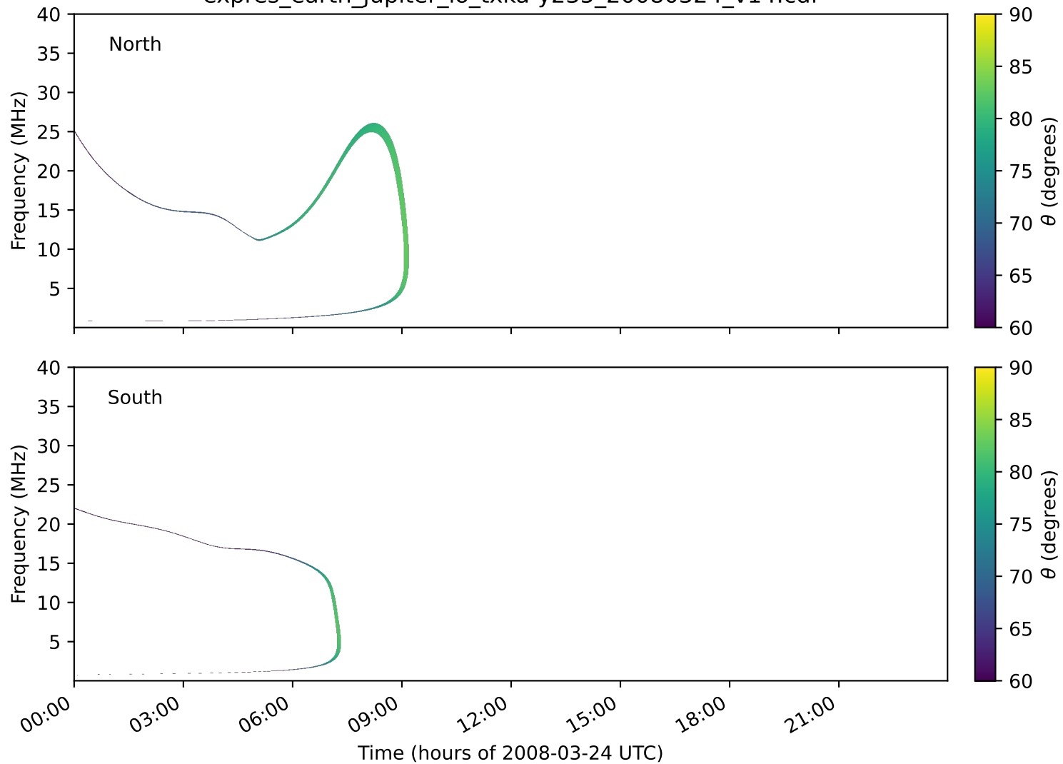
expres_earth_jupiter_io_txka-y235_20080324_v14.cdf
