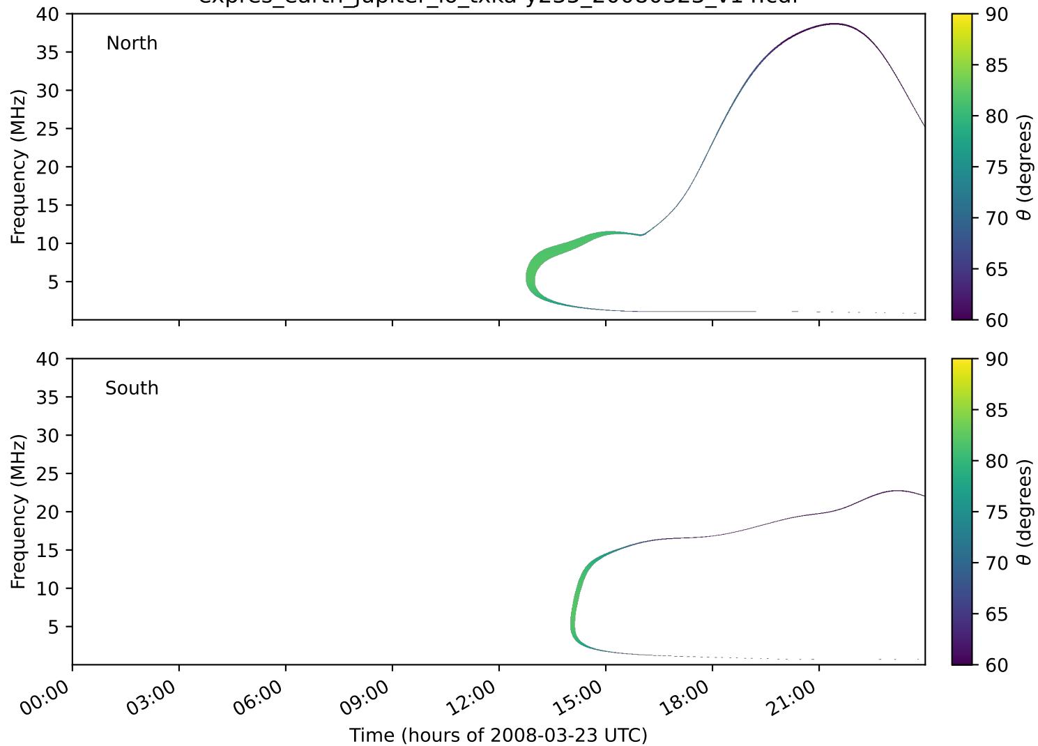
expres_earth_jupiter_io_txka-y235_20080323_v14.cdf
