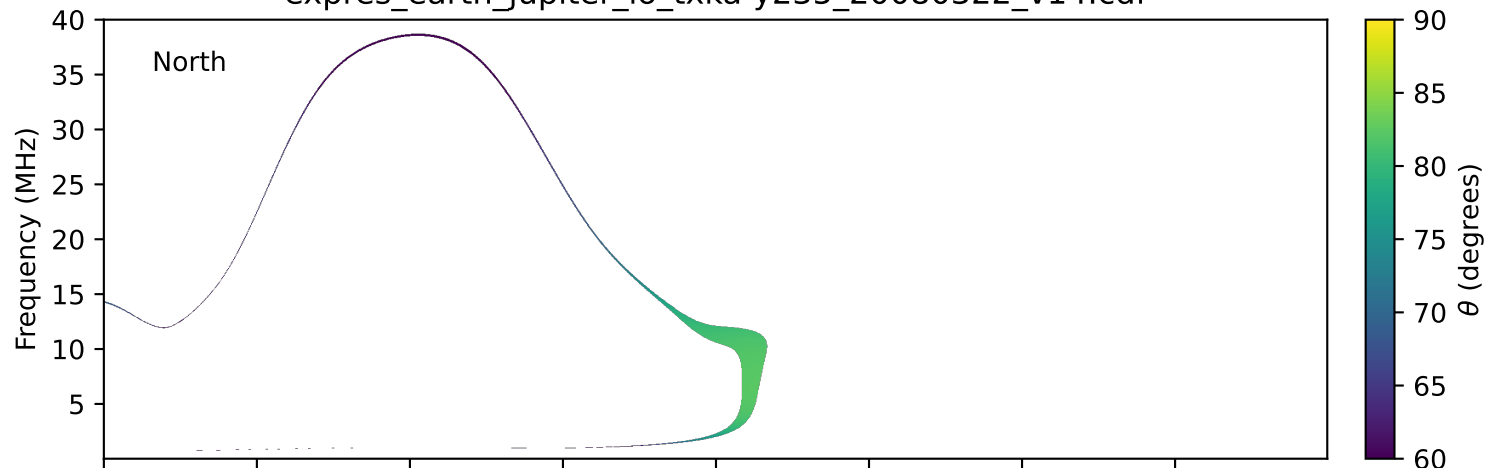
expres_earth_jupiter_io_txka-y235_20080322_v14.cdf
