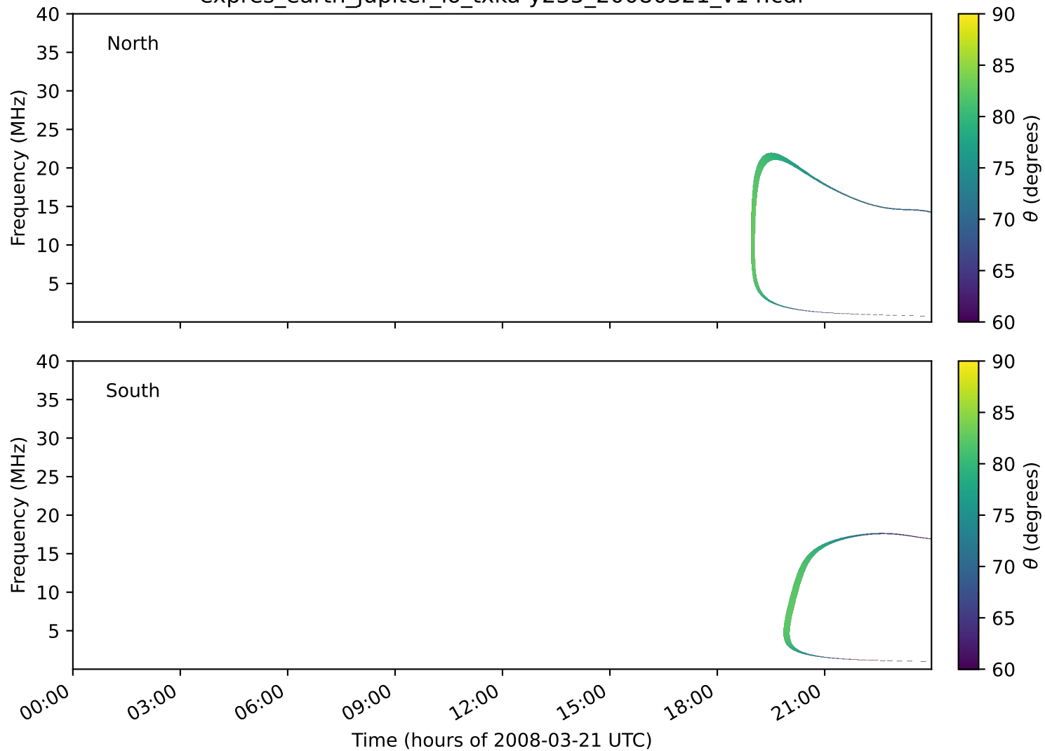
expres_earth_jupiter_io_txka-y235_20080321_v14.cdf
