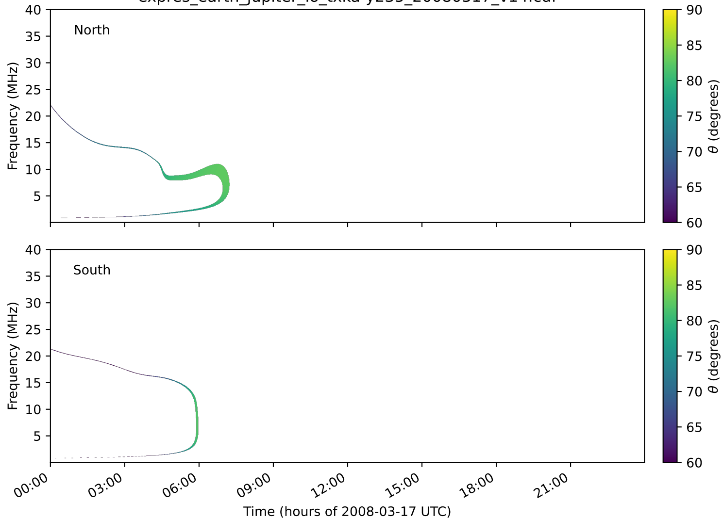
expres_earth_jupiter_io_txka-y235_20080317_v14.cdf
