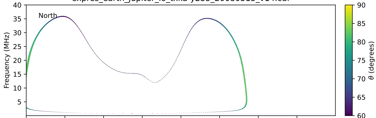
expres_earth_jupiter_io_txka-y235_20080313_v14.cdf
