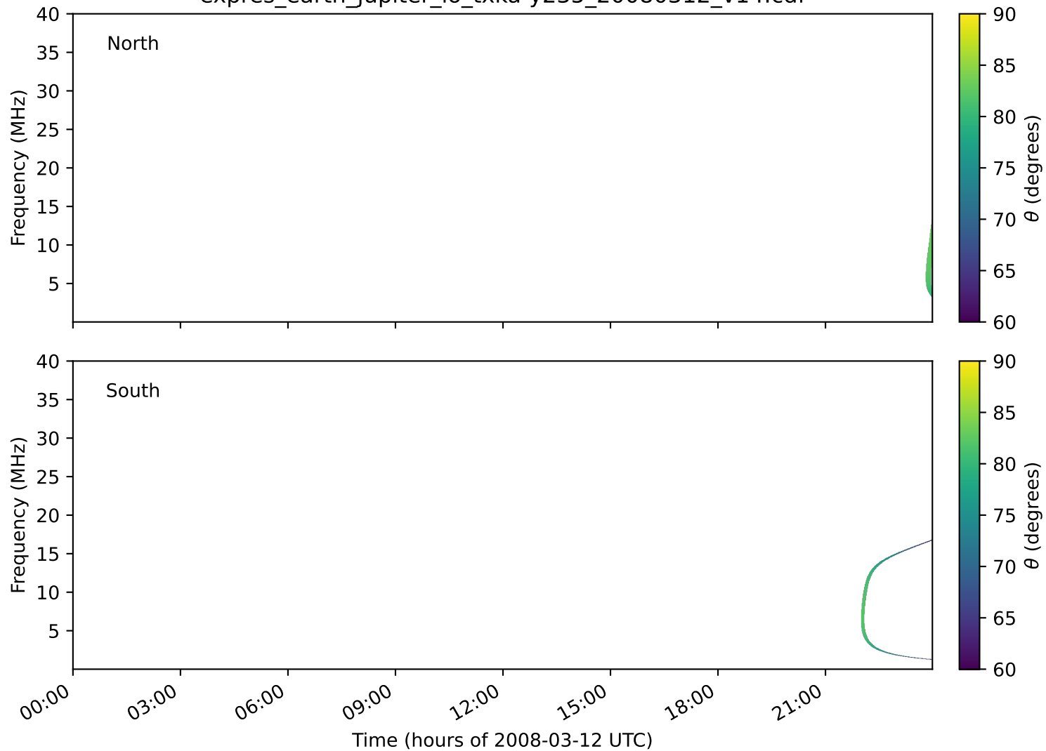
expres_earth_jupiter_io_txka-y235_20080312_v14.cdf
