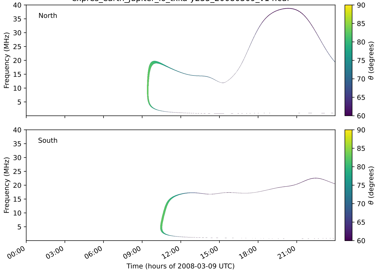
expres_earth_jupiter_io_txka-y235_20080309_v14.cdf
